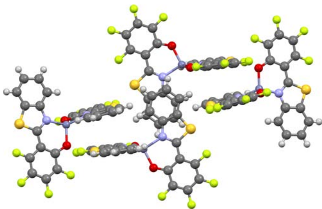
Figure 3. Intermolecular contacts in the crystal structure of 19 , showing \pi_{\text{H}}-\pi_{\text{H}} and \pi_{\text{F}}-\pi_{\text{F}} stacking.
